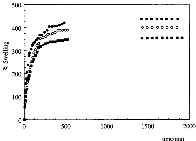
FIGURE 4. Swelling curves of AAm/CA hydrogels containing 1 M Dalapon: and 1% BDMA. Given total dose is 5.2 kGy: ● 40 mg CA; ○ 20mg CA; ■ 0 mg CA.
